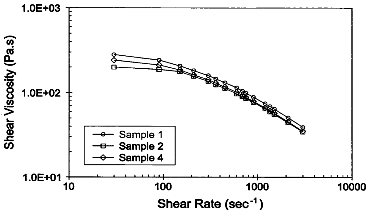
Fig. 11 Shear Viscosity of Plasticized Metallocene Propylene Homopolymers
